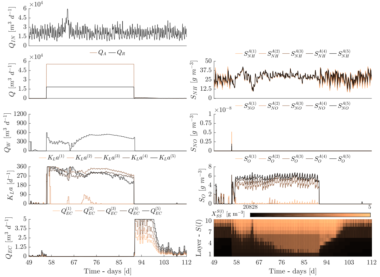
Figure 9.7: Case II, t \in [49, 112] : Influent flow-rate Q_{IN} , flow-rates ( Q_A, Q_R, Q_W ), oxygen transfer coefficients K_La^{(1 \sim 5)} , and extra carbon flow-rates Q_{EC}^{(1 \sim 5)} , left panels, together with nitrogen forms S_{NH}^{A(1 \sim 5)} and S_{NO}^{A(1 \sim 5)} , soluble oxygen S_O^{A(1 \sim 5)} , and total suspended solids X_{SS}^{S(1 \sim 10)} , right panels.
