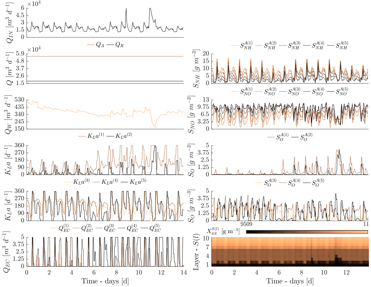
Figure 8.6: Treatment control, MPC: Influent flow-rate Q_{IN} , flow-rates ( Q_A, Q_R, Q_W ), oxygen transfer coefficients K_{La}^{(1\sim 5)} , and extra carbon flow-rates Q_{EC}^{(1\sim 5)} , left panels, together with nitrogen forms S_{NH}^{A(1\sim 5)} and S_{NO}^{A(1\sim 5)} , soluble oxygen S_O^{A(1\sim 5)} , and total suspended solids X_{SS}^{S(1\sim 10)} , right panels.
