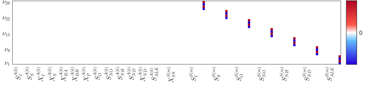
Figure 7.5: Pair (A^{SS}, B^{SS}) : Eigenvectors \nu_i(\lambda_i) for \lambda_i \in \sigma(A^{SS}) with \text{rank}([\lambda_i I - A^{SS} \ B^{SS}]) < N_x .
