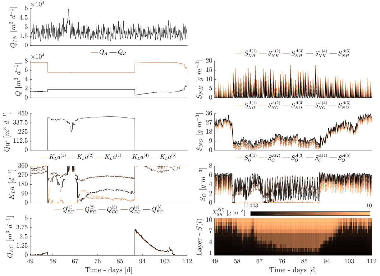
Figure 9.5: Case I, t \in [49, 112] : Influent flow-rate Q_{IN} , flow-rates ( Q_A, Q_R, Q_W ), oxygen transfer coefficients K_{La}^{(1 \sim 5)} , and extra carbon flow-rates Q_{EC}^{(1 \sim 5)} , left panels, together with nitrogen forms S_{NH}^{A(1 \sim 5)} and S_{NO}^{A(1 \sim 5)} , soluble oxygen S_O^{A(1 \sim 5)} , and total suspended solids X_{SS}^{S(1 \sim 10)} , right panels.
