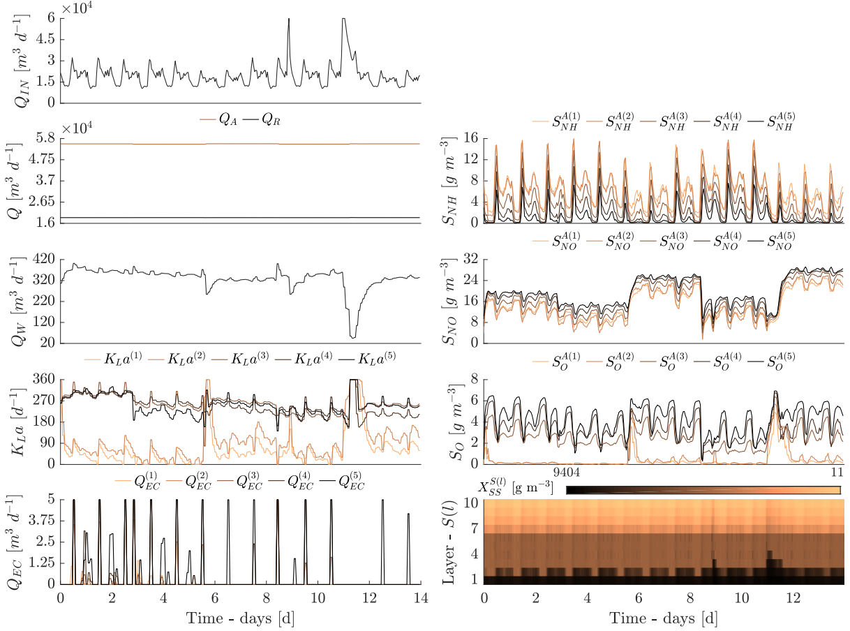
Figure 9.2: Reuse, MPC: Influent flow-rate Q_{IN} , flow-rates ( Q_A, Q_R, Q_W ), oxygen transfer coefficients K_{La}^{(1\rightsquigarrow 5)} , and extra carbon flow-rates Q_{EC}^{(1\rightsquigarrow 5)} , left panels, together with nitrogen forms S_{NH}^{A(1\rightsquigarrow 5)} and S_{NO}^{A(1\rightsquigarrow 5)} , soluble oxygen S_O^{A(1\rightsquigarrow 5)} , and total suspended solids X_{SS}^{S(1\rightsquigarrow 10)} , right panels.
