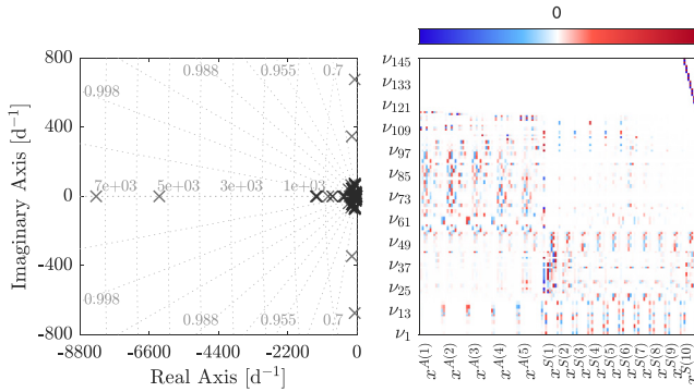
Fig. 7. Spectrum \sigma(A^{SS}) : Eigenvalues \lambda_i \in \sigma(A^{SS}) and associated eigenvectors v_i(\lambda_i) (left and right panels, respectively). The grid in the complex plane displays lines corresponding to constant damping factors (diagonal lines) and natural frequencies (vertical lines, in rad/days) for the associated modes.
