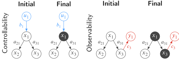
Fig. 3. Example 3.1: The colouring procedure applied to the subgraphs \mathcal{G}_c = (\mathcal{V}_c, \mathcal{E}_c) , left, and \mathcal{G}_o = (\mathcal{V}_o, \mathcal{E}_o) , right. As not all nodes x_{n_x} \in \mathcal{V}_A can be coloured black, neither graph is colourable and the system (A, B, C) is thus uncontrollable and unobservable in a strong structural sense, an expected result. Note that augmenting the state-space with a control u_2 (respectively, a sensor y_2 ) acting on (measuring) state-variable x_2 leads to a strongly structural controllable (observable) system.
