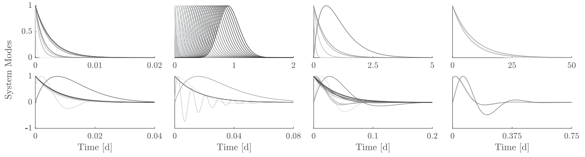
Fig. 8. The normalised modes t^k e^{\lambda_i t} / \max_t t^k e^{\lambda_i t} ( k = 0, \dots, \mu(\lambda_i) - 1 ) for the real eigenvalues (top) and complex conjugated pairs of eigenvalues (bottom) from the spectrum \sigma(A^{SS}) = \{\lambda_i, v_i(\lambda_i)\}_{i=1}^{N_k} . Grouping is based on each mode's time constant \tau_i = 1/\text{Re}[\lambda_i] .
