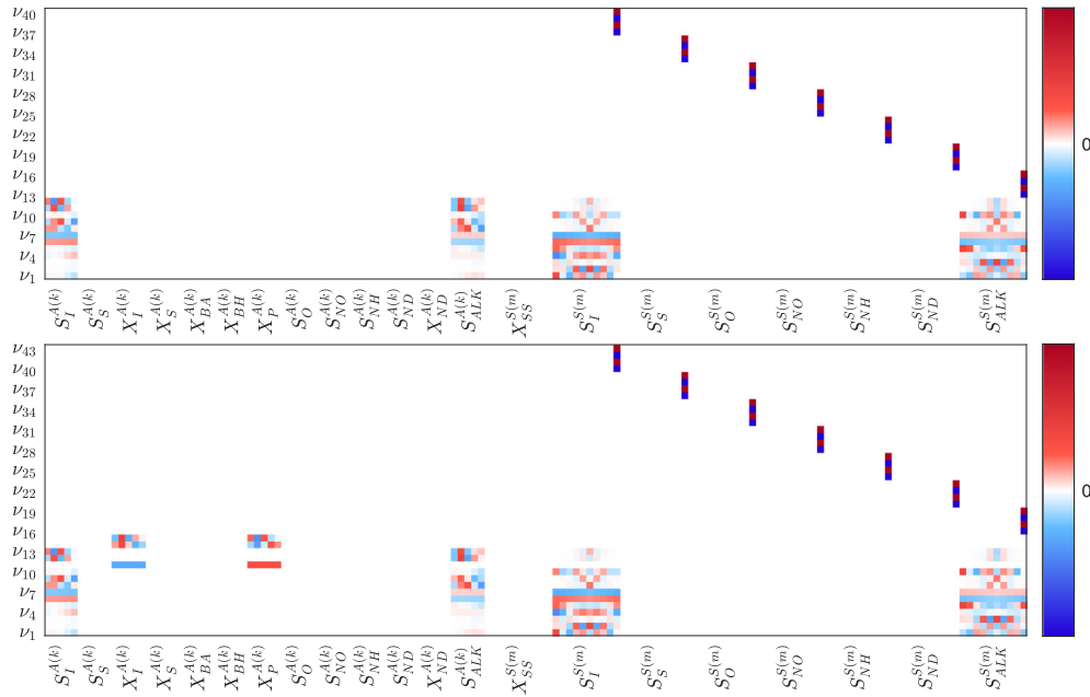
Fig. 14. System (A_d^{SS}, B_d^{SS}, C_d^{SS}) : Eigenvectors v_i(\lambda_i) associated with \lambda_i \in \sigma(A_d^{SS}) failing the PBH controllability test ( \text{rank}([\lambda_i I - A_d^{SS} B_d^{SS}]) < N_x ), top, and with \lambda_i \in \sigma(A_d^{SS}) failing the PBH observability test ( \text{rank}([\lambda_i I - A_d^{SS} C_d^{SS}]^T) < N_x ), bottom.
