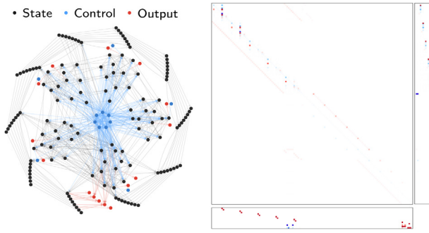
Fig. 6. Network \mathcal{G}_{SS} = (\mathcal{V}_{SS}, \mathcal{E}_{SS}) (left) associated to linearisation (A^{SS}, B^{SS}, C^{SS}) (right). State vertices x_{n_x} \in \mathcal{V}_{AS} and state-state edges (x_{n_x}, x_{n'_x}) \in \mathcal{E}_{AS} are in black, input vertices u_{n_u} \in \mathcal{V}_{BS} and input-state edges (u_{n_u}, x_{n_x}) \in \mathcal{E}_{BS} are in blue, and output vertices y_{n_y} \in \mathcal{V}_{CS} and state-output edges (x_{n_x}, y_{n_y}) \in \mathcal{E}_{CS} are in red. State self-loops have been omitted.
