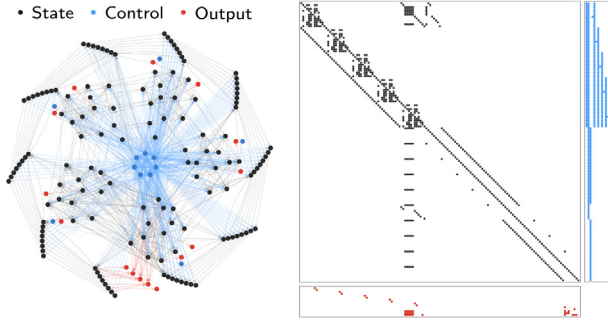
Fig. 4. Network \mathcal{G} = (\mathcal{V}, \mathcal{E}) (left) for structured system (A, B, C) (right). State vertices x_{n_x} \in \mathcal{V}_A are in black, input vertices u_{n_u} \in \mathcal{V}_B in blue, and output vertices y_{n_y} \in \mathcal{V}_C in red. State-state (x_{n_x}, x_{n'_x}) \in \mathcal{E}_A , input-state (u_{n_u}, x_{n_x}) \in \mathcal{E}_B , and state-output edges (x_{n_x}, y_{n_y}) \in \mathcal{E}_C are dyed to match the corresponding entries in (A, B, C) . Self-loops have been omitted.
