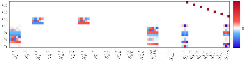
Fig. 12. Pair (A_s^{SS}, C_s^{SS}) : Eigenvectors v_i(\lambda_i) with \lambda_i \in \sigma(A_s^{SS}) failing the PBH observability test ( \text{rank}([ \lambda_i I - A_s^{SS \top} \ C_s^{SS \top} ]^\top) < N_x ).
