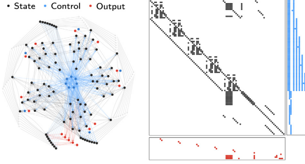
Fig. 11. Network \mathcal{G}_s = (\mathcal{V}_s, \mathcal{E}_s) (left) associated to (A_s, B_s, C_s) (right). State vertices x_{n_x} \in \mathcal{V}_{A_s} are in black, input vertices u_{n_u} \in \mathcal{V}_{B_s} are in blue, and output vertices y_{n_y} \in \mathcal{V}_{C_s} are in red. State-state edges (x_{n_x}, x_{n'_x}) \in \mathcal{E}_{A_s} , input-state edges (u_{n_u}, x_{n_x}) \in \mathcal{E}_{B_s} , and state-output edges (x_{n_x}, y_{n_y}) \in \mathcal{E}_{C_s} are dyed to match the corresponding entries in (A_s, B_s, C_s) . Self-loops are omitted.
