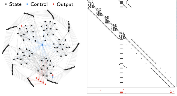
Fig. 13. Network \mathcal{G}_d = (\mathcal{V}_d, \mathcal{E}_d) associated to (A_d, B_d, C_d) (left and right panels, respectively). State vertices x_{n_x} \in \mathcal{V}_A are in black, input vertices u_{n_u} \in \mathcal{V}_B are in blue, and output vertices y_{n_y} \in \mathcal{V}_C are in red. State-state edges (x_{n_x}, x_{n'_x}) \in \mathcal{E}_A , input-state edges (u_{n_u}, x_{n_x}) \in \mathcal{E}_B , and state-output edges (x_{n_x}, y_{n_y}) \in \mathcal{E}_C are dyed to match the corresponding entries in (A_d, B_d, C_d) . The state self-loops have been omitted.
