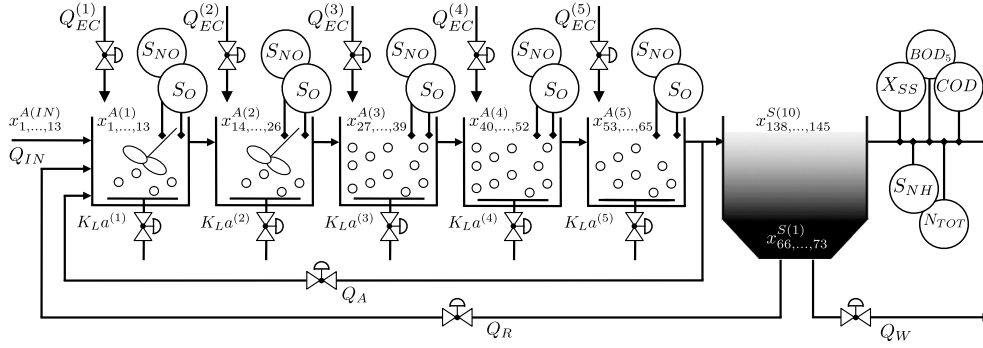
Fig. 1. The activated sludge plant: Process layout.
