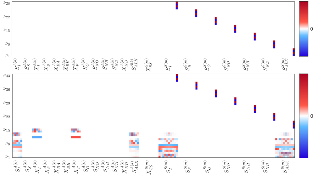
Fig. 9. System (A^{SS}, B^{SS}, C^{SS}) : Eigenvectors v_i(\lambda_i) associated with eigenvalues \lambda_i \in \sigma(A^{SS}) failing the PBH controllability test ( \text{rank}([\lambda_i I - A^{SS} \ B^{SS}]) < N_x ), top; and \lambda_i \in \sigma(A^{SS}) failing the PBH observability test ( \text{rank}([\lambda_i I - A^{SS \top} \ C^{SS \top}]^T) < N_x ), bottom.
