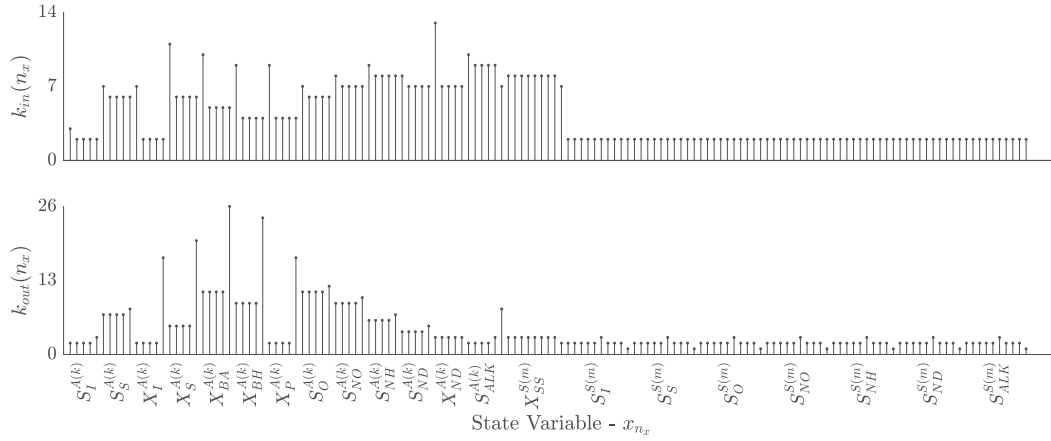
Fig. 5. Network \mathcal{G} = (\mathcal{V}, \mathcal{E}) : In-degree, k_{in}(n_x) , and out-degree, k_{out}(n_x) , centralities associated to each state node x_{n_x} \in \mathcal{V}_A .
