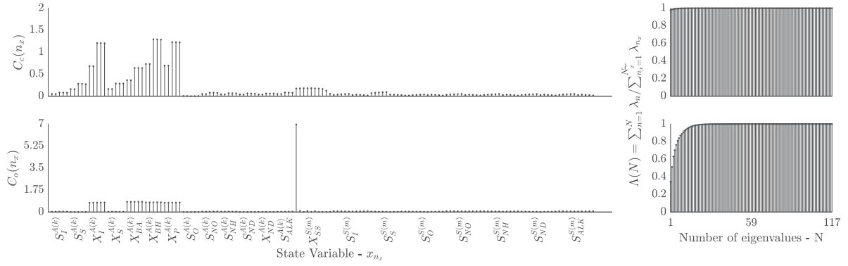
Fig. 10. System (A^{SS}, B^{SS}, C^{SS}) : On the left, the average controllability centrality C_c(n_x) , top, and average observability centrality C_o(n_x) , bottom, associated to each state variable x_{n_x} ( n_x = 1, \dots, N_x ). On the right, the cumulative sum \Lambda(N) for the eigenvalues of the infinite-horizon controllability Gramian W_c(\infty) , top, and the infinite-horizon observability Gramian W_o(\infty) , bottom.
