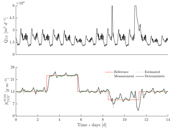
Fig. 3. Influent flow-rate Q_{IN} , top, and reference tracking of effluent total nitrogen N_{TOT}^{S(10)} , bottom.
